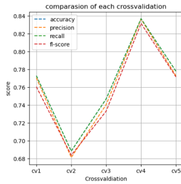
Figure 8. Performance Graph of Manhattan Distance K-Fold 5
