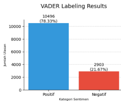
Figure 3 VADER Labeling Result
