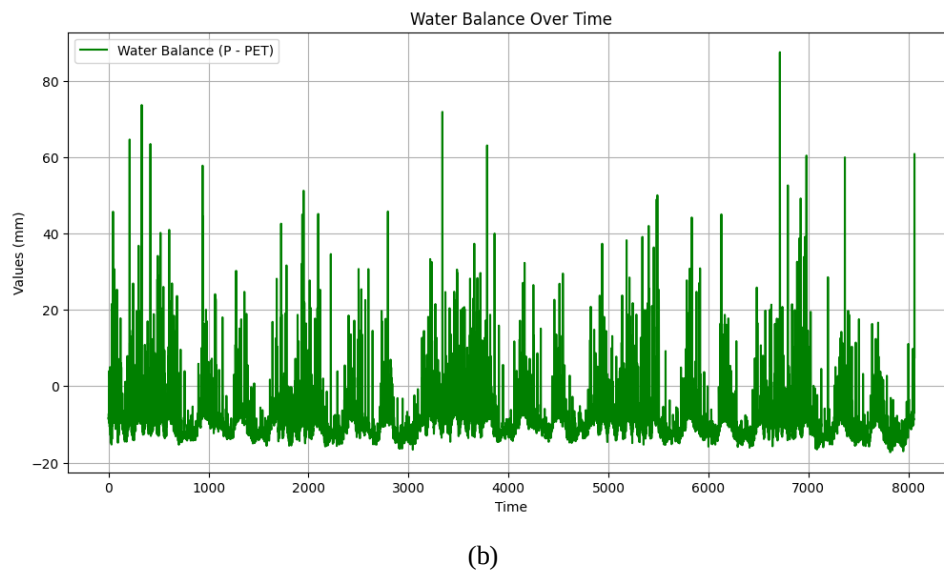
Figure 4. (a) Daily potential evapotranspiration (PET) and (b) Water balance over the study period.
