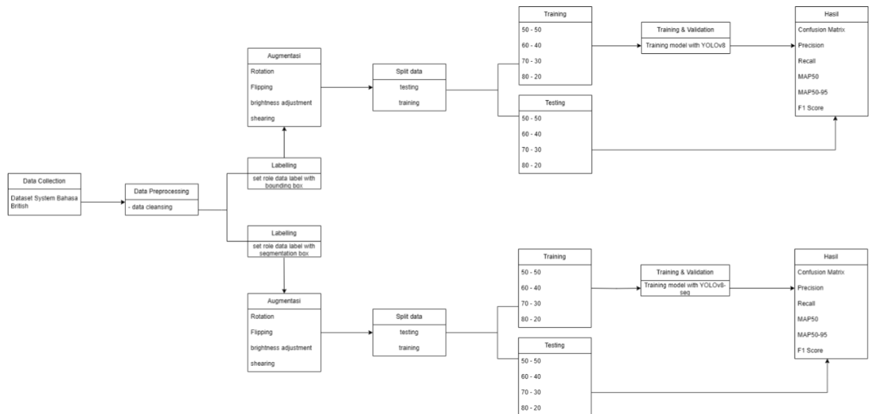
Figure 1. Research Flowchart
