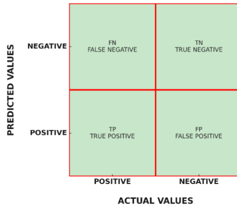
Figure 5. Confusion Matrix
