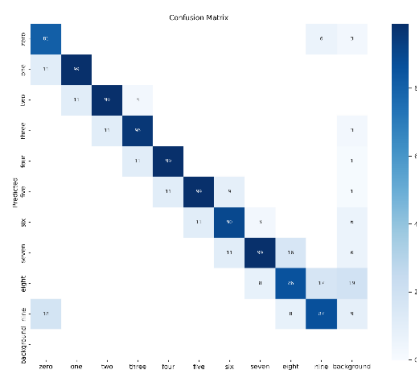
Figure 4. Confusion Matrix
