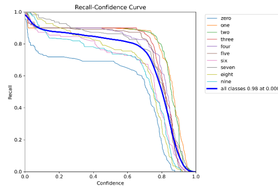
Figure 9. Recall-Confidence Curve
