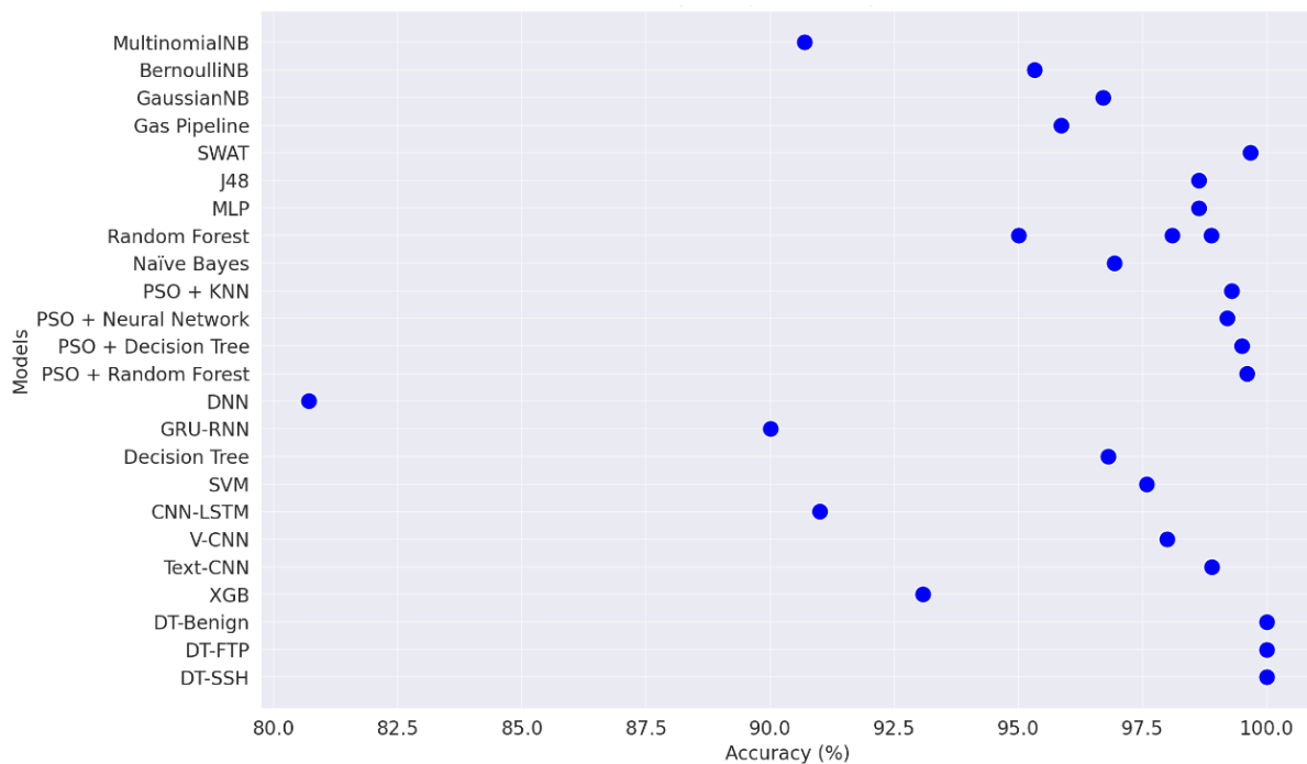
Figure 5. Accuracy Performance Across Model
