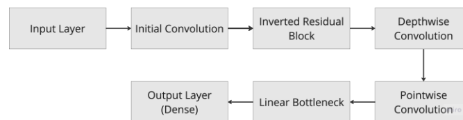
Figure 3. MobileNetV2 Architecture
