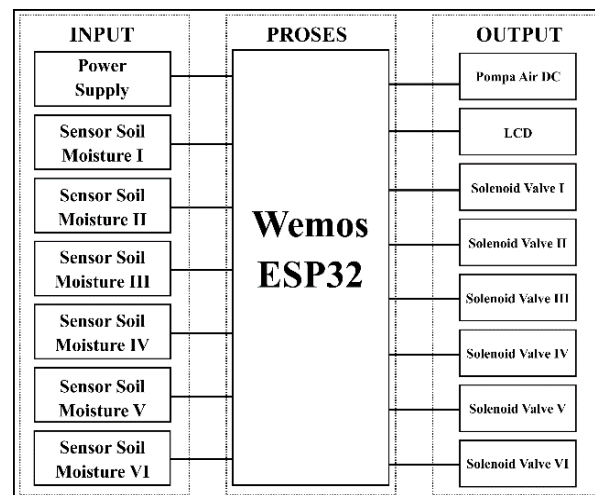
Figure 2. Diagram Block
