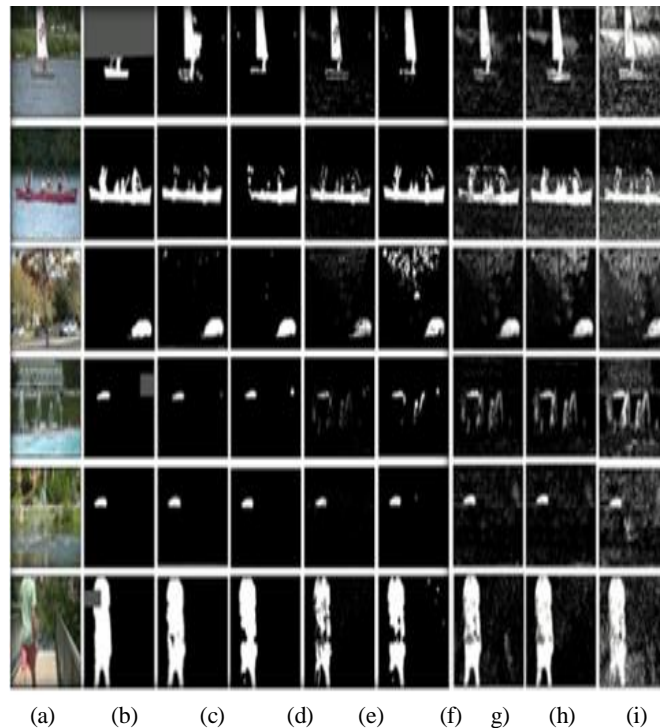
Figure 4. The visual comparison (a) original scene (b) ground-truth (c) The proposed FCM-CS foreground mask (d) SuBSENSE foreground mask (e) ViBe foreground mask (f) LOBSTER foreground mask (g) GMM foreground mask (h) KNN foreground mask (i) Codebook foreground mask
