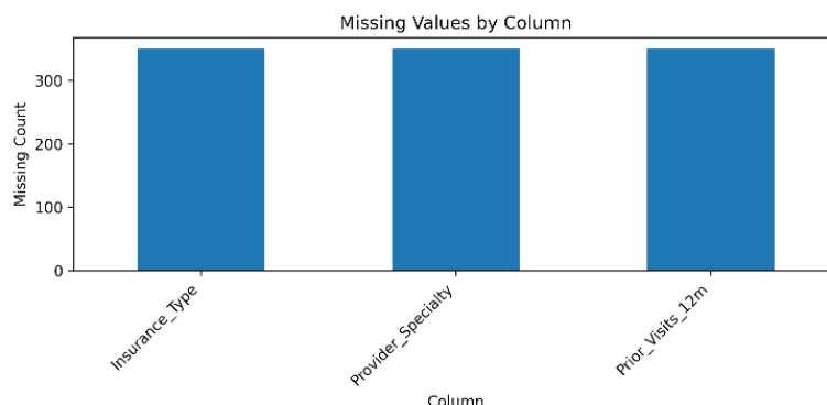
Figure 2. Missing values by column
