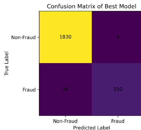
Figure 3. Confusion matrix of the best model
