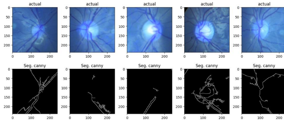
Figure 3: Class Normal
