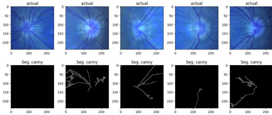
Figure 5: Class Pseudopapilledema
