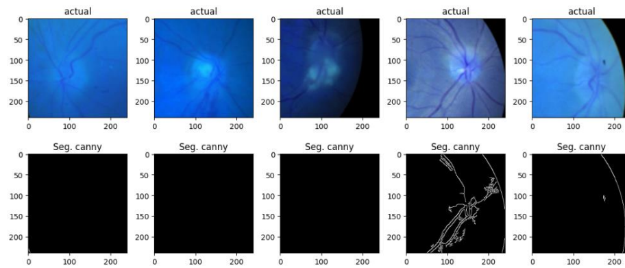
Figure 4: Class Papilledema
