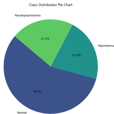
Figure 2: Class Distribution
